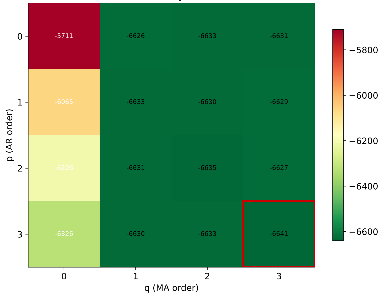
AIC Heatmap — d = 1
