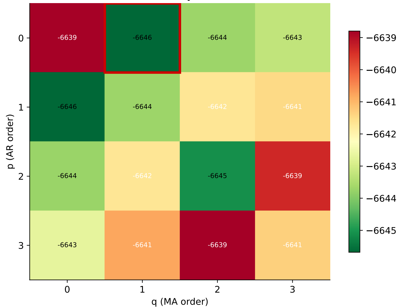
AIC Heatmap — d = 0
