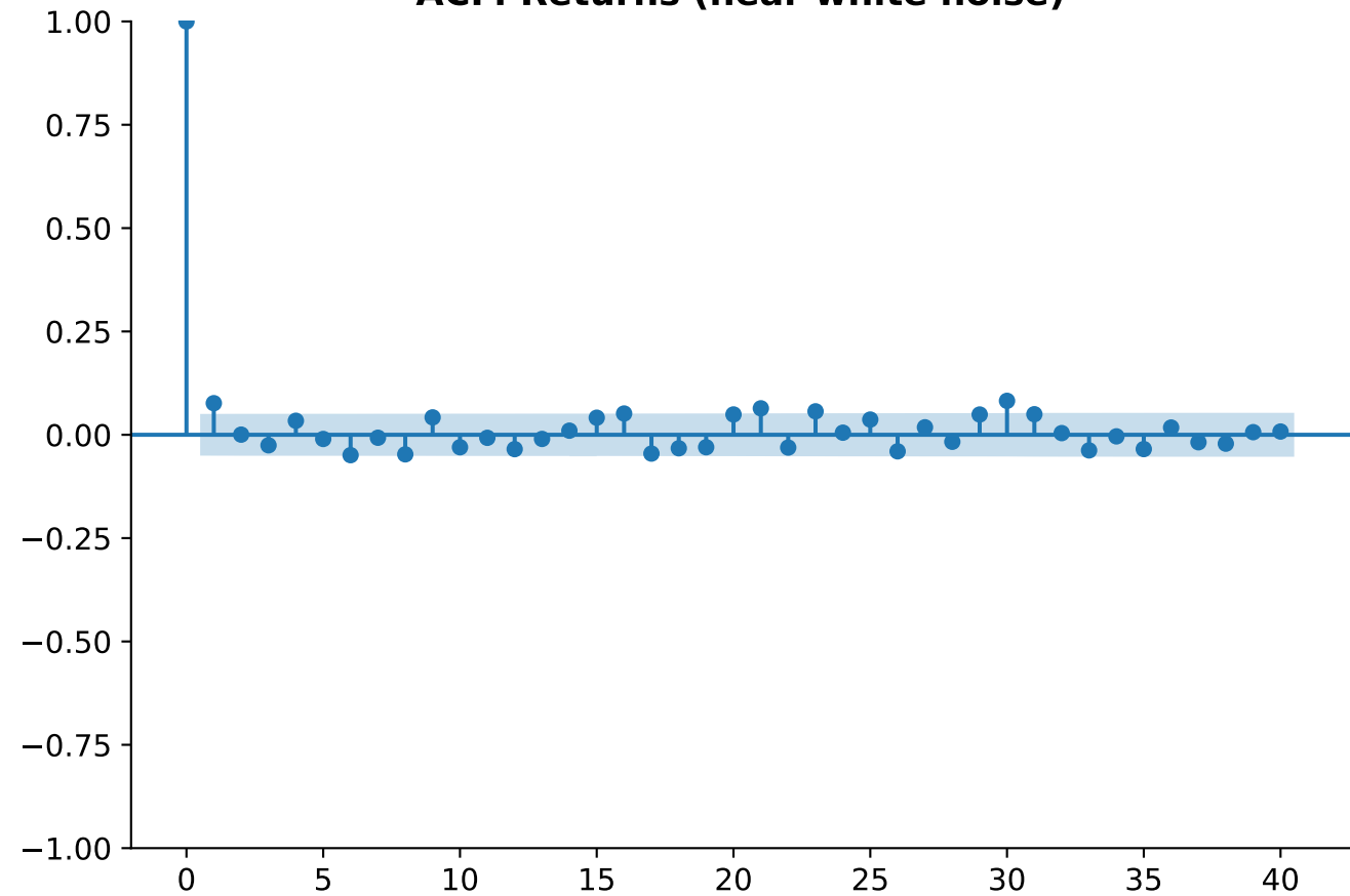
ACF: Returns (near white noise)
