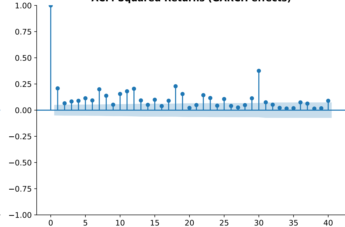
ACF: Squared Returns (GARCH effects)
