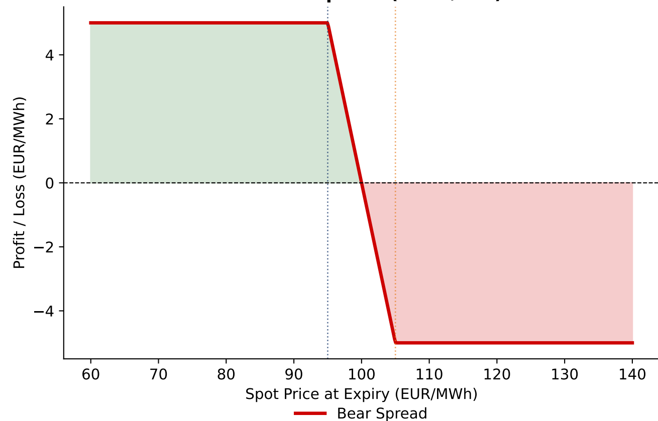
Bear Put Spread (K=95/105)
