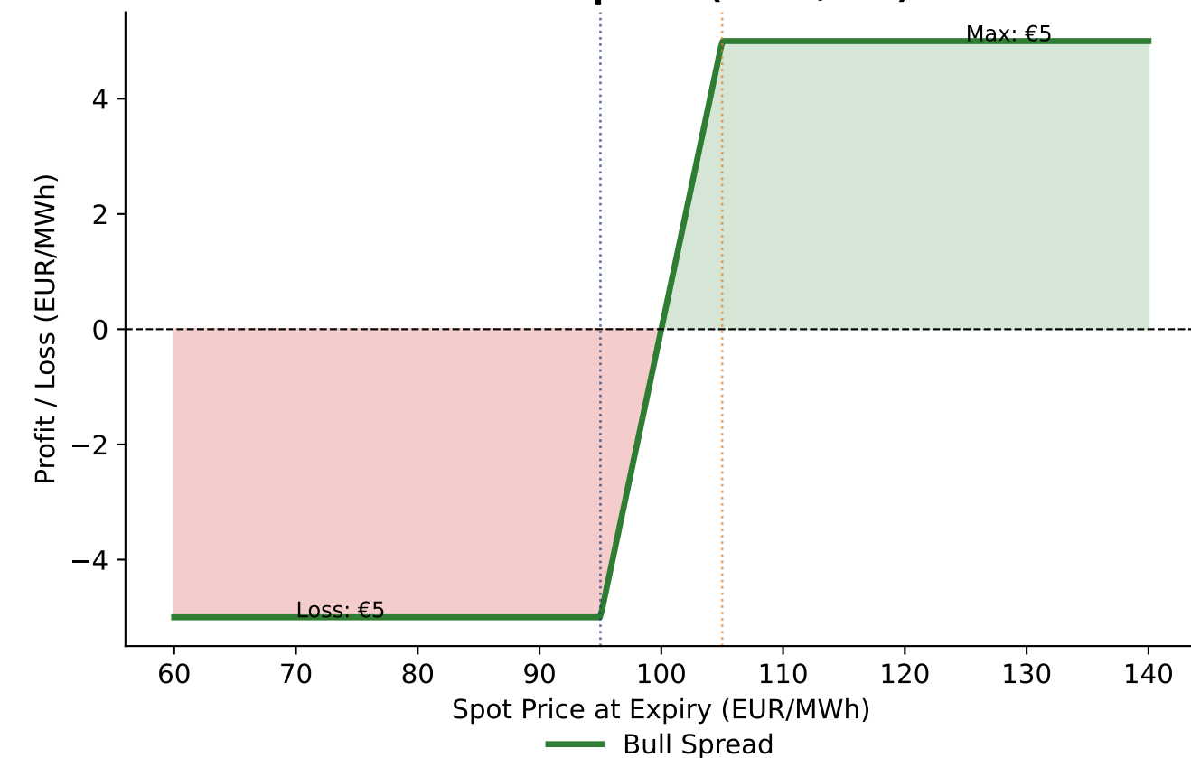
Bull Call Spread (K=95/105)
