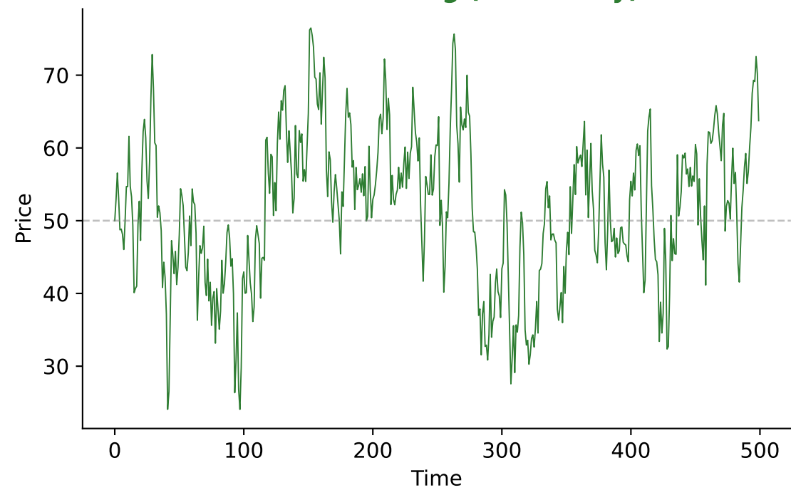
Mean-Reverting (Stationary)
