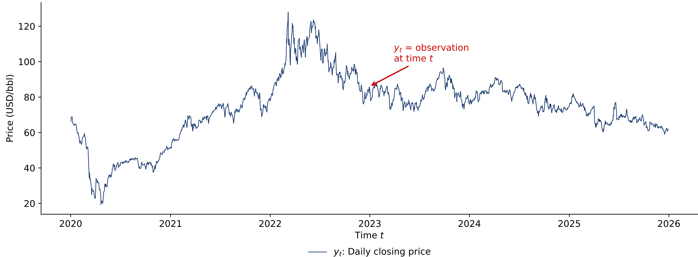
A Time Series: Brent Crude Oil \{y_t : t = 1, \dots, T\}
