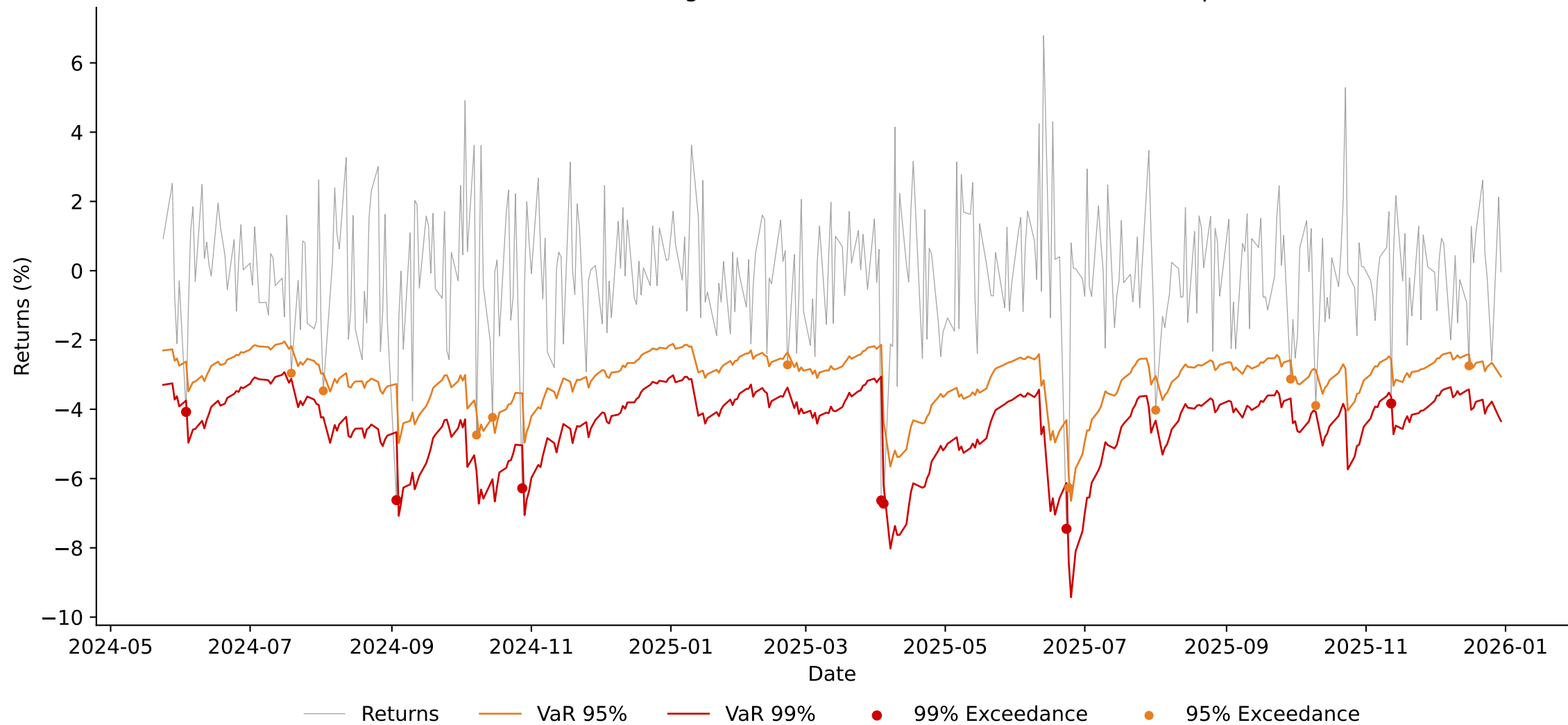
VaR Backtest — Rolling GARCH(1,1) on Brent Crude (Out-of-Sample)
