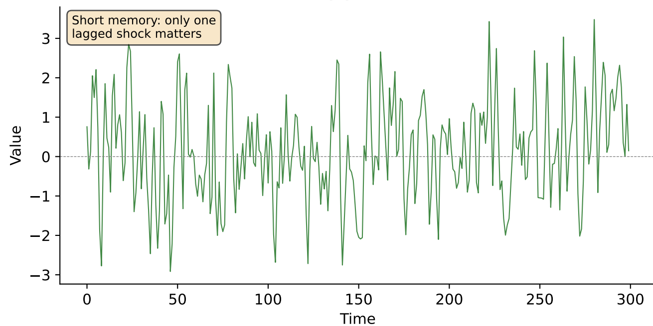
MA(1) \theta = 0.8
