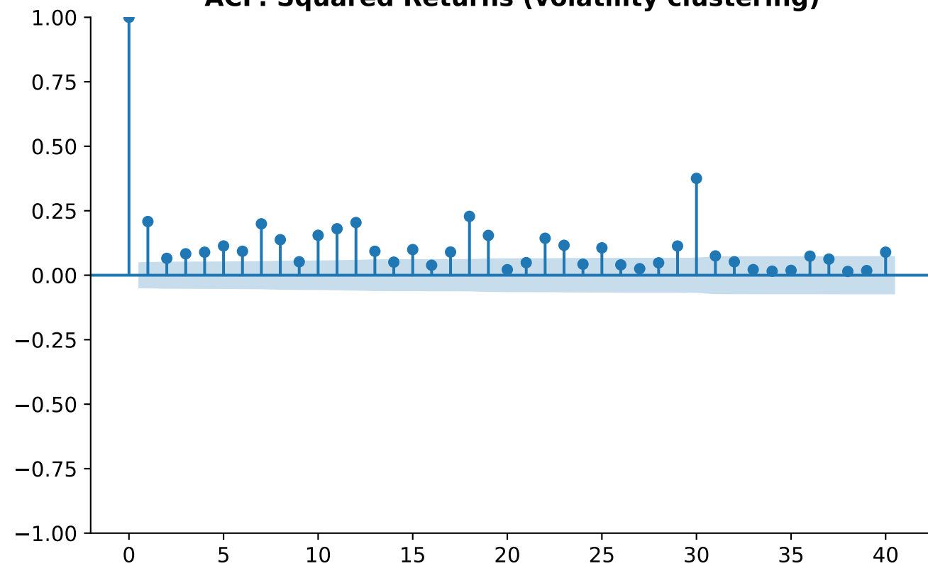
ACF: Squared Returns (volatility clustering)
