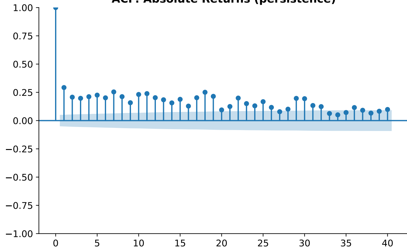
ACF: Absolute Returns (persistence)
