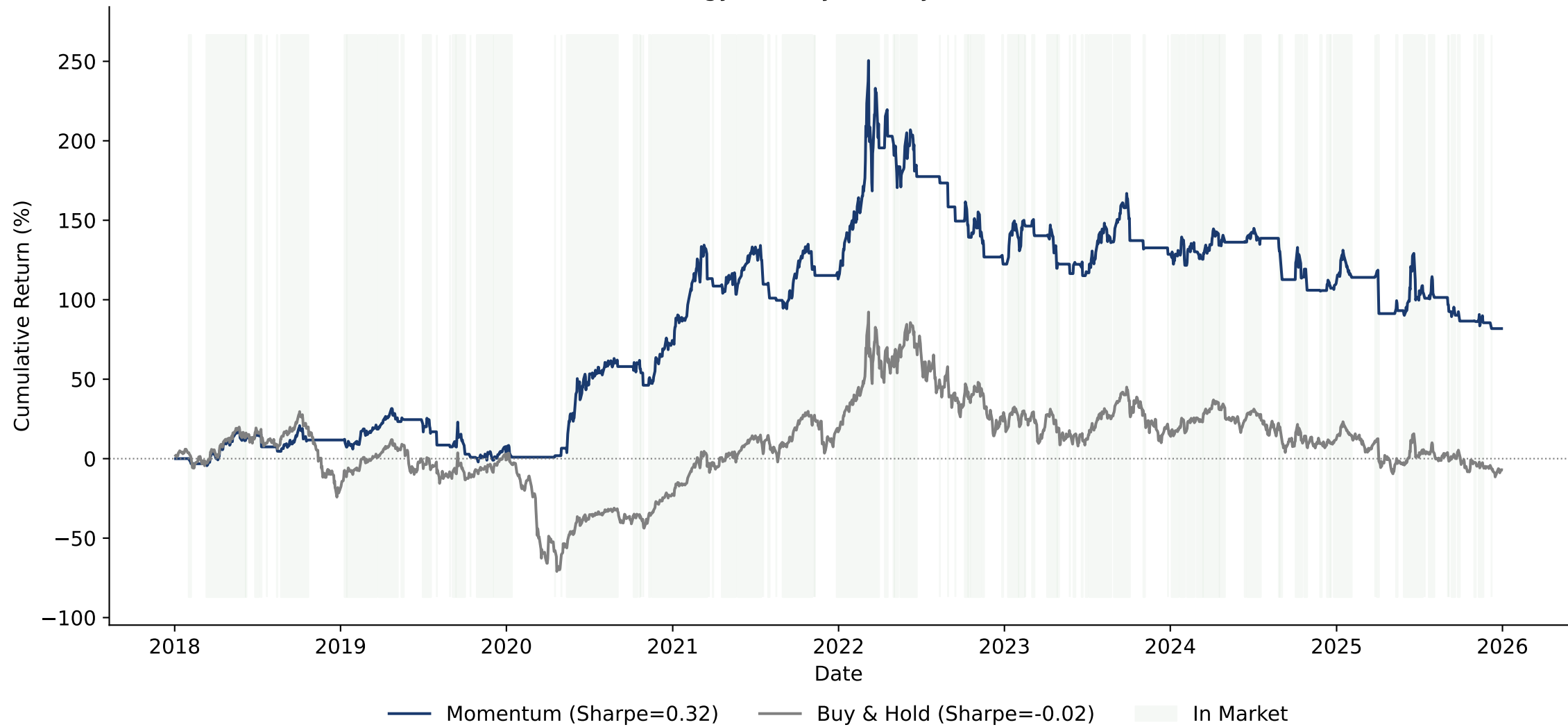
Momentum Strategy (20-day) vs Buy & Hold - Brent Crude
