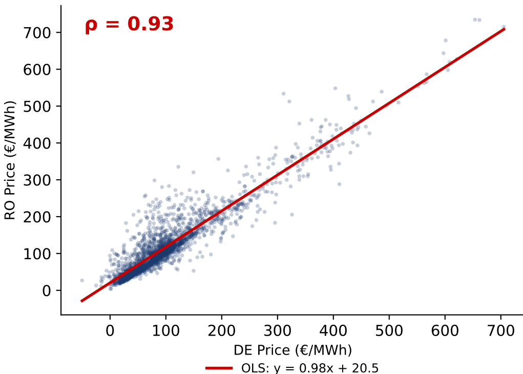
Scatter: RO vs DE Prices
