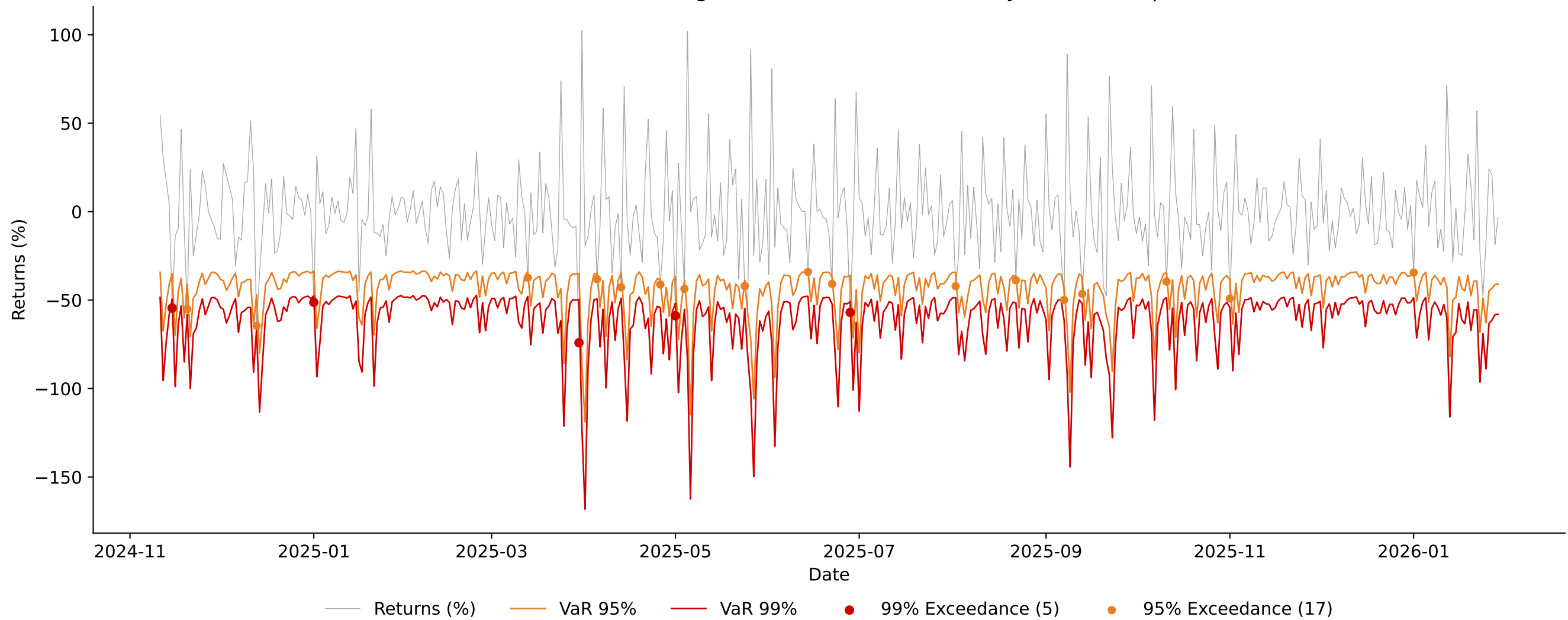
VaR Backtest — Rolling GARCH(1,1) on RO Electricity (Out-of-Sample)
