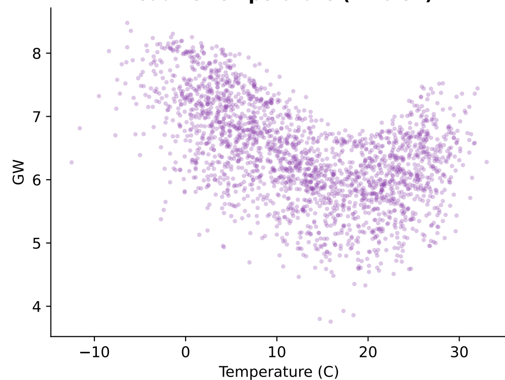
Load vs Temperature ( r=-0.51 )
