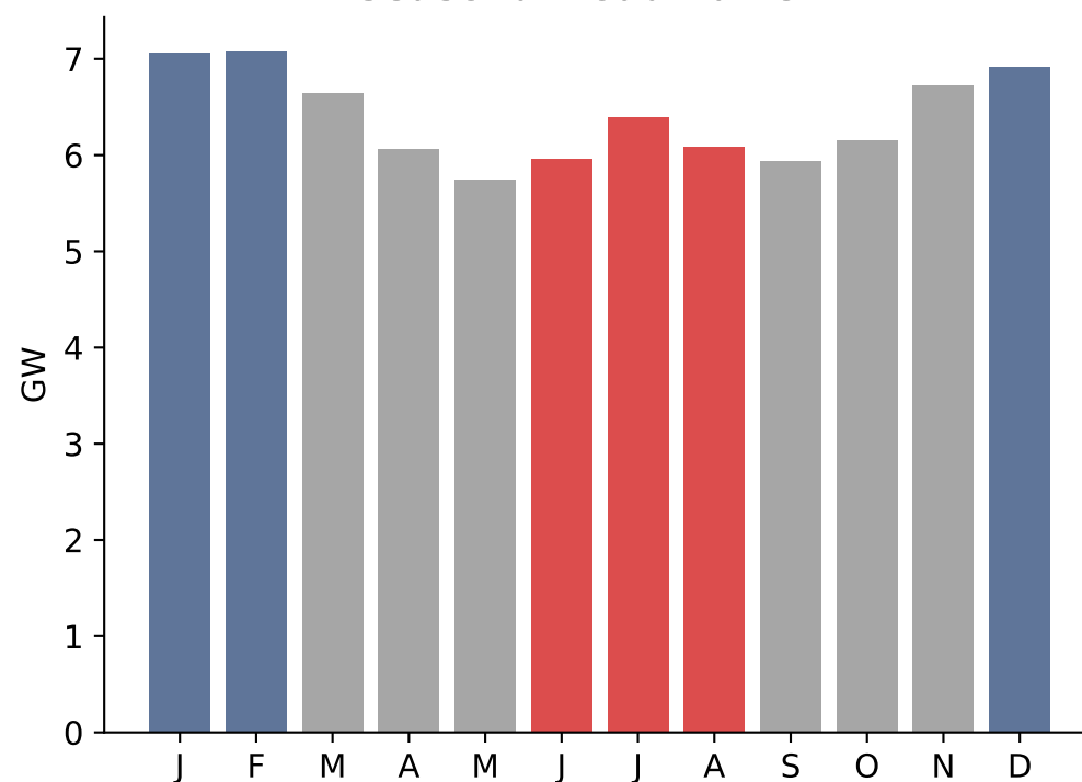
Seasonal Load Pattern
