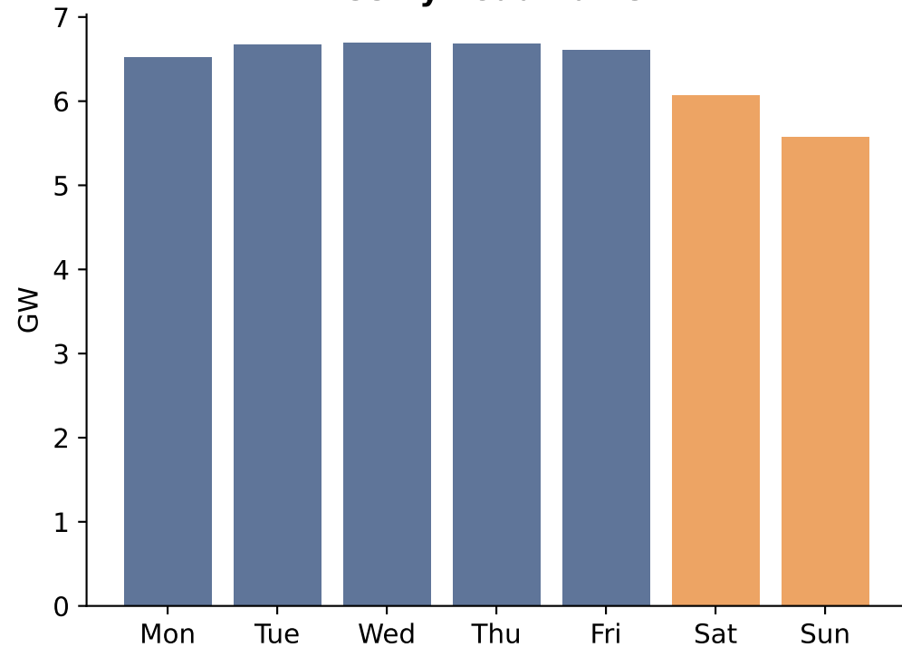
Weekly Load Pattern
