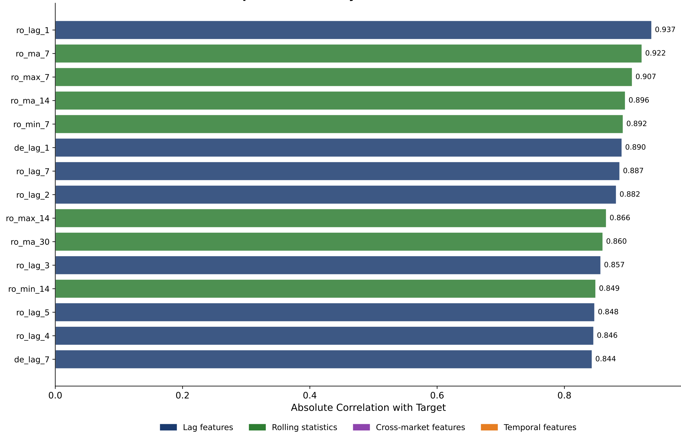
Top 15 Features by Correlation with Price
