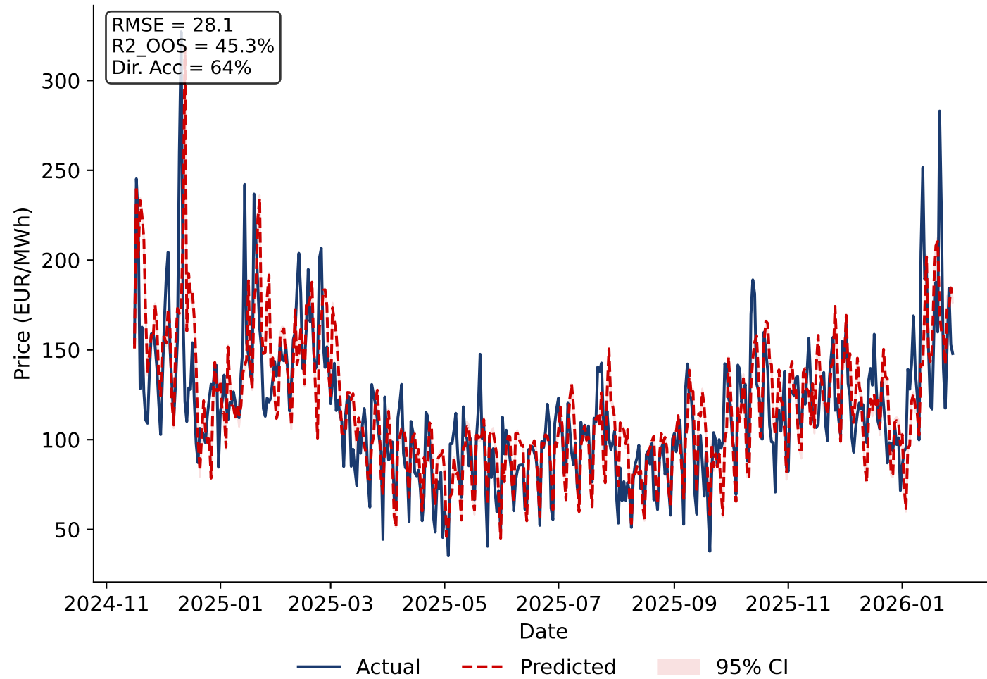
Test Set: Gradient Boosting Forecast
