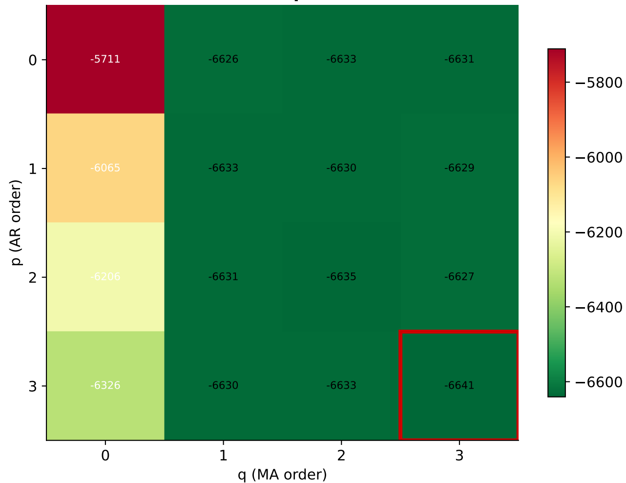
AIC Heatmap — d = 1
