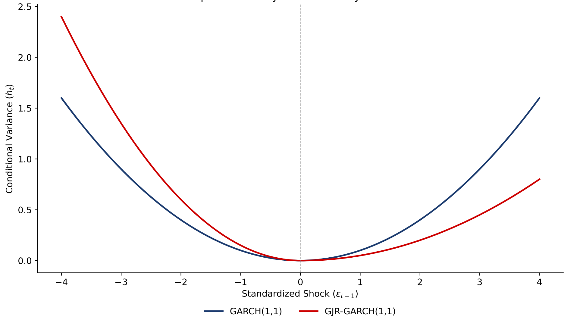
News Impact Curve: Symmetric vs Asymmetric GARCH
