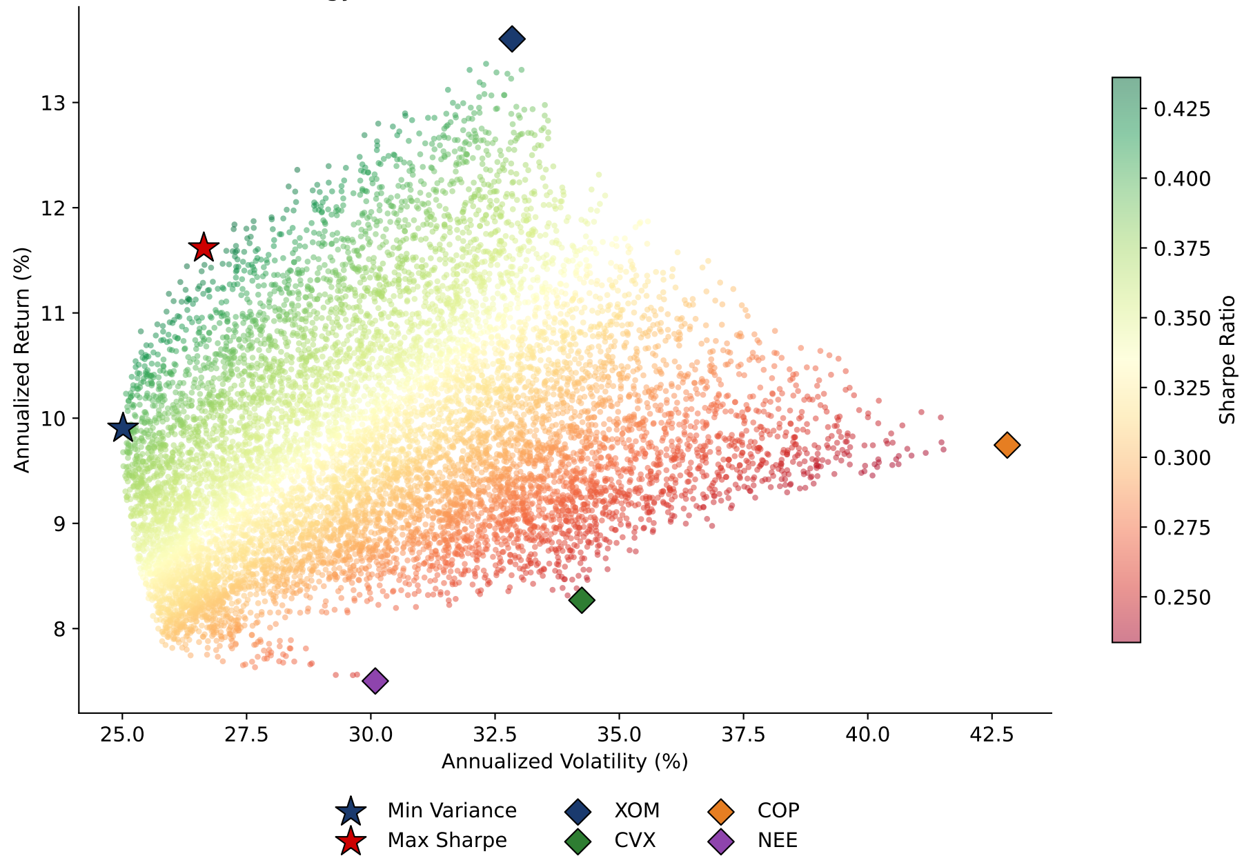
Energy Portfolio - Efficient Frontier (Monte Carlo)
