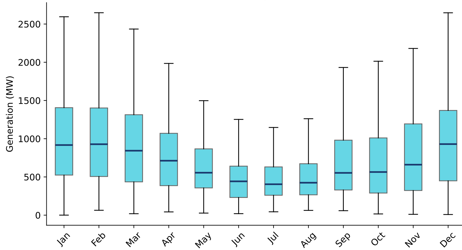
(C) Wind by Month
