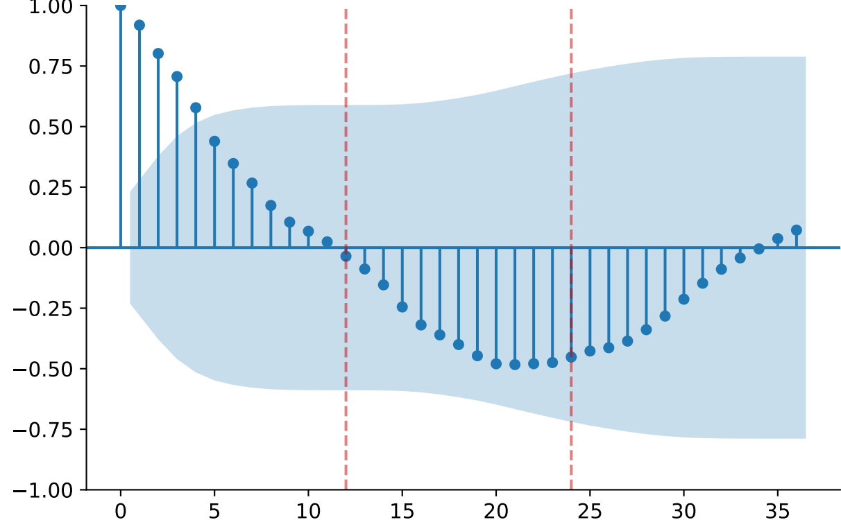
ACF: Monthly Gas (spikes at lag 12, 24)
