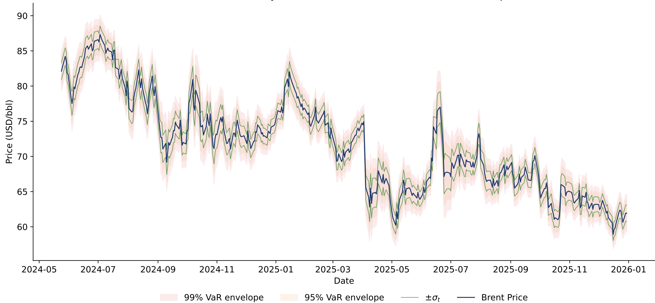
GARCH(1,1) Volatility and VaR Bands — Brent Crude (Out-of-Sample)
