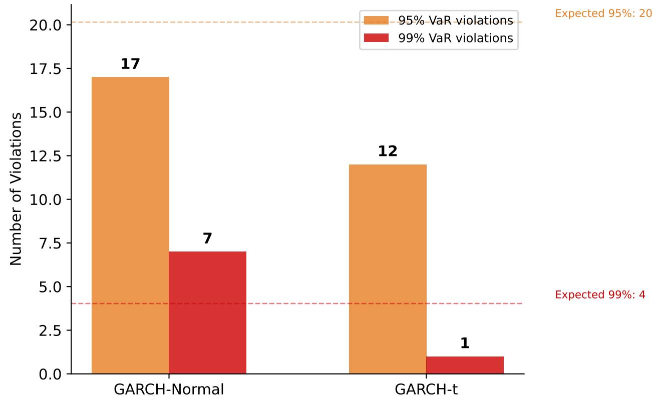
(A) VaR Violations
