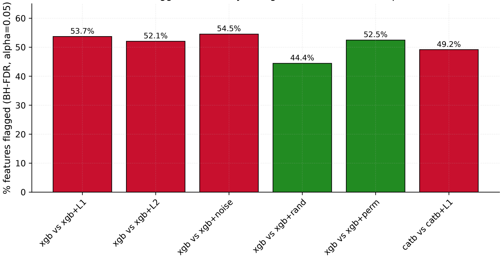
BH-flagged fraction by configuration (block-bootstrap)
