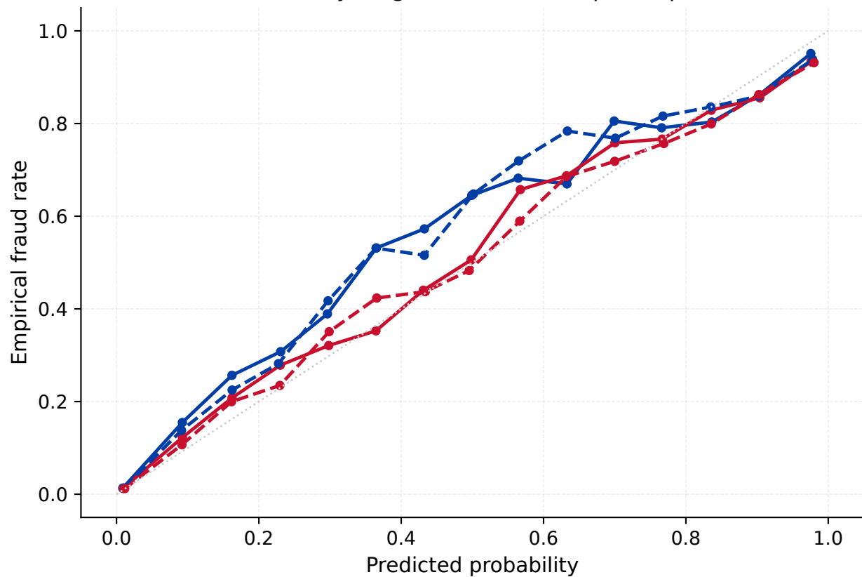
Reliability diagrams on the temporal split
