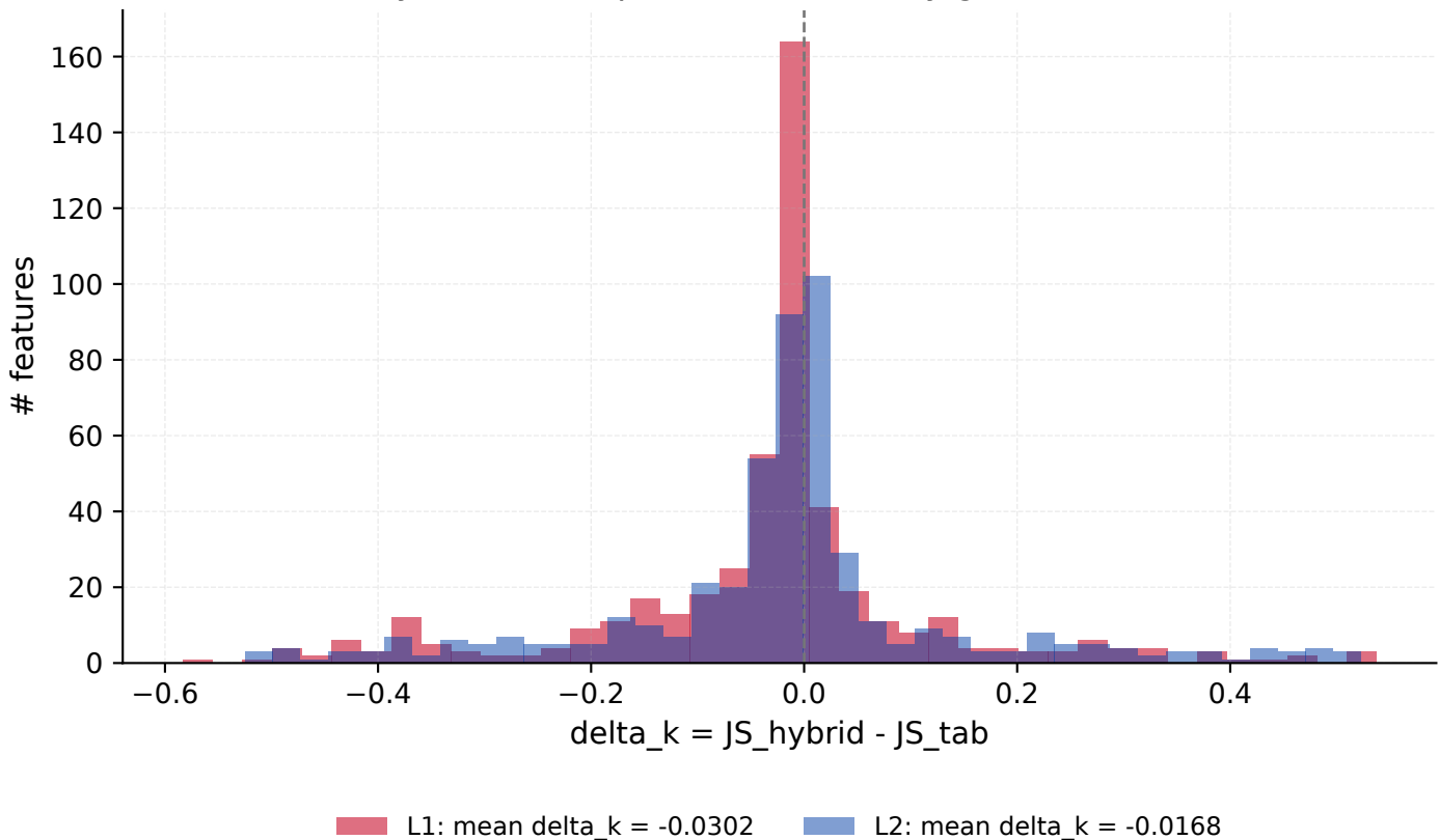
Layer ablation: per-feature stability gain (L1 vs L2)
