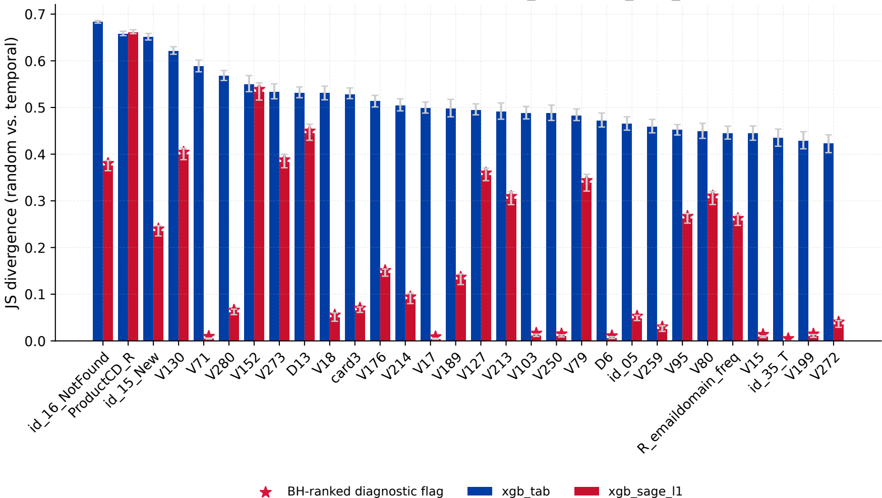
Top 30 most unstable features: xgb_tab vs. xgb_sage_l1
