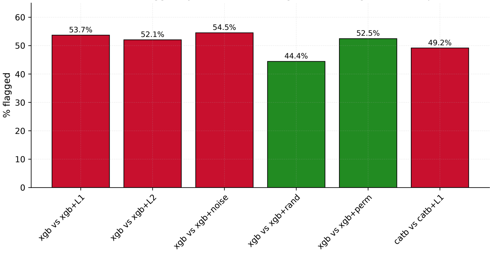
Fraction of features flagged by the BH-ranked diagnostic, read against the empirical null
