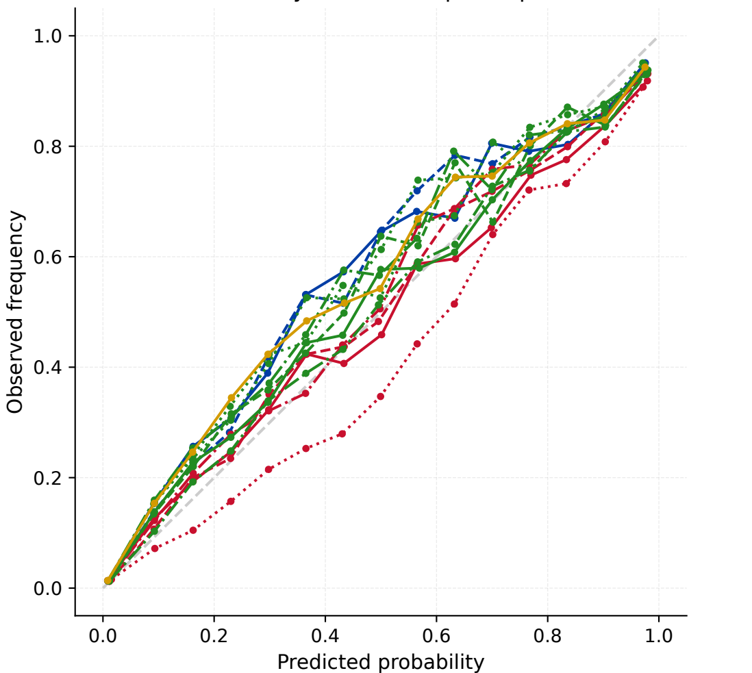
Reliability curves (temporal split)
