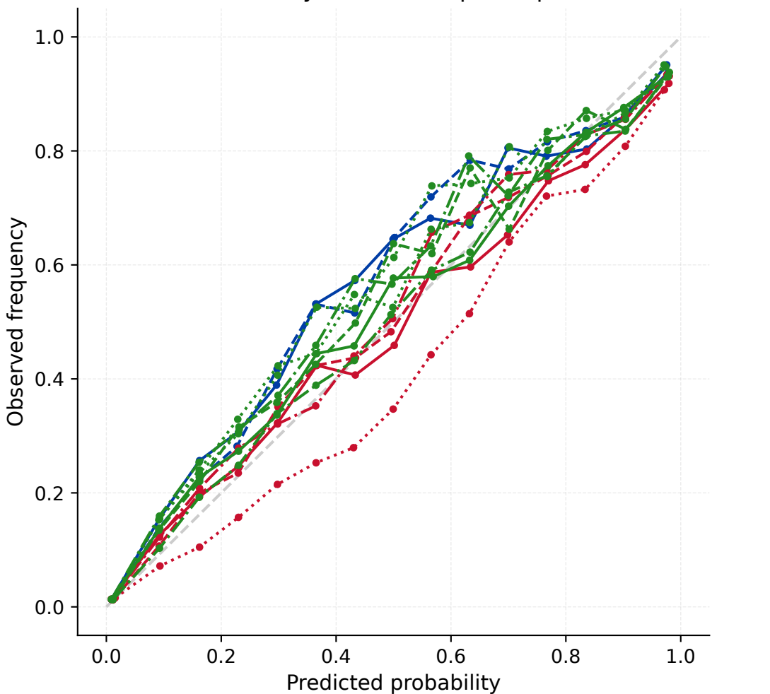
Reliability curves (temporal split)
