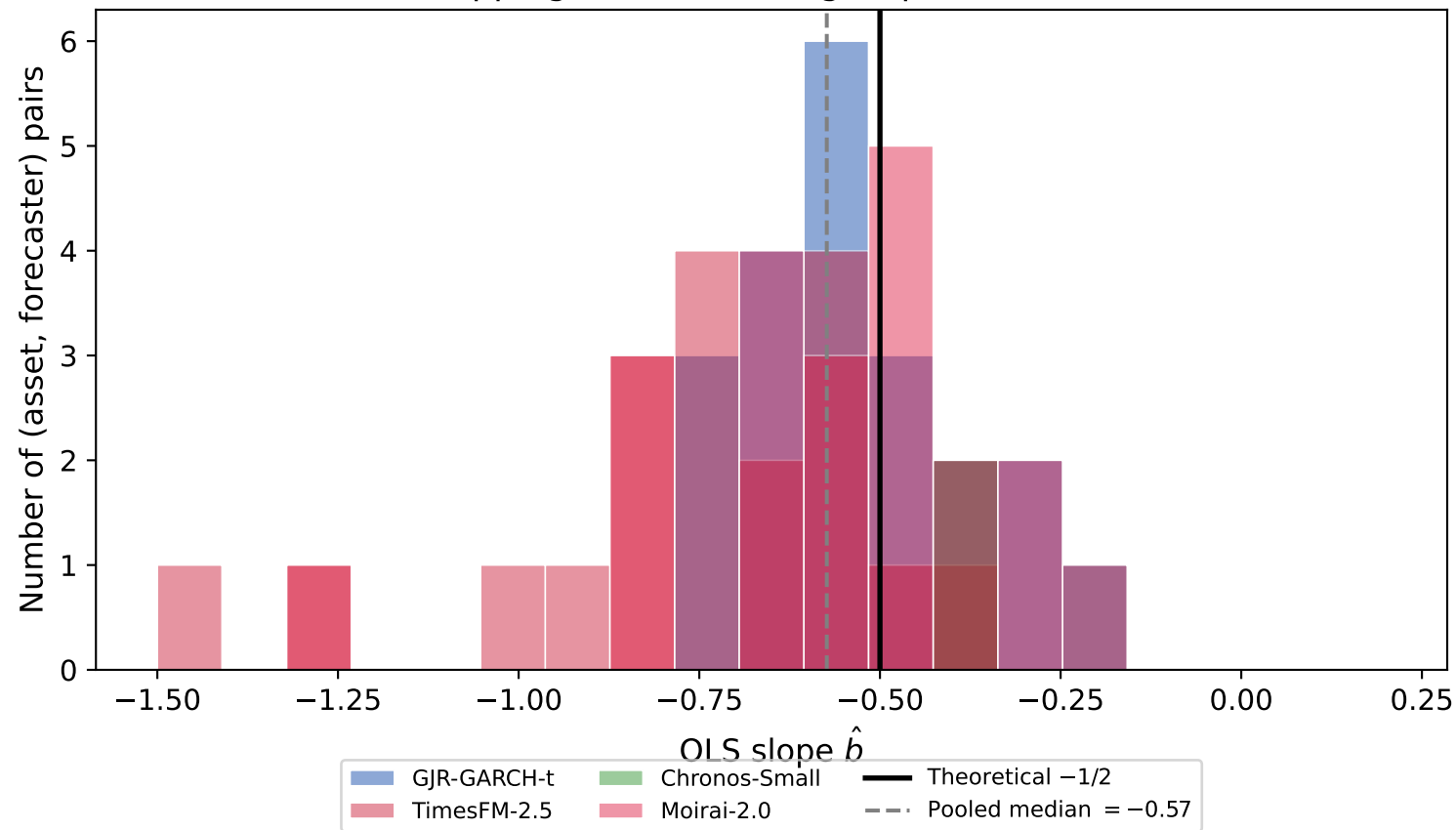
Non-overlapping window scaling slopes — all forecasters
