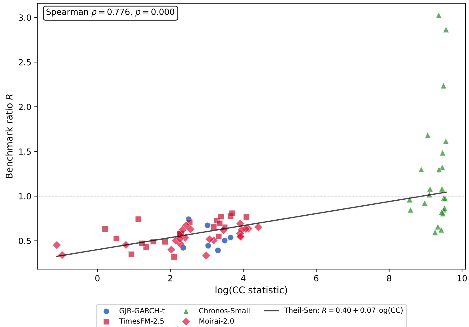
Christoffersen CC statistic vs. benchmark ratio ( \alpha = 1\% )
