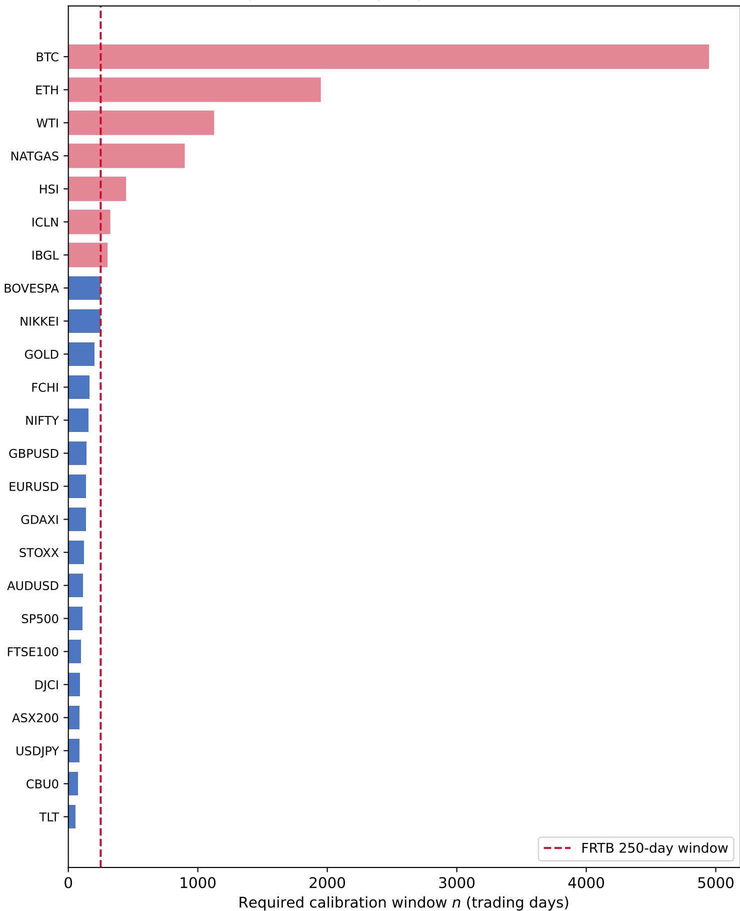
Required n for 50 bp ES precision at \alpha = 2.5\%
