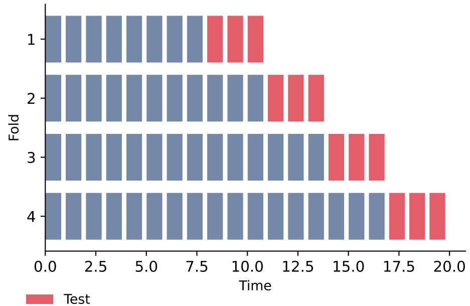
Rolling Origin CV (CORRECT) Always train on past, test on future
