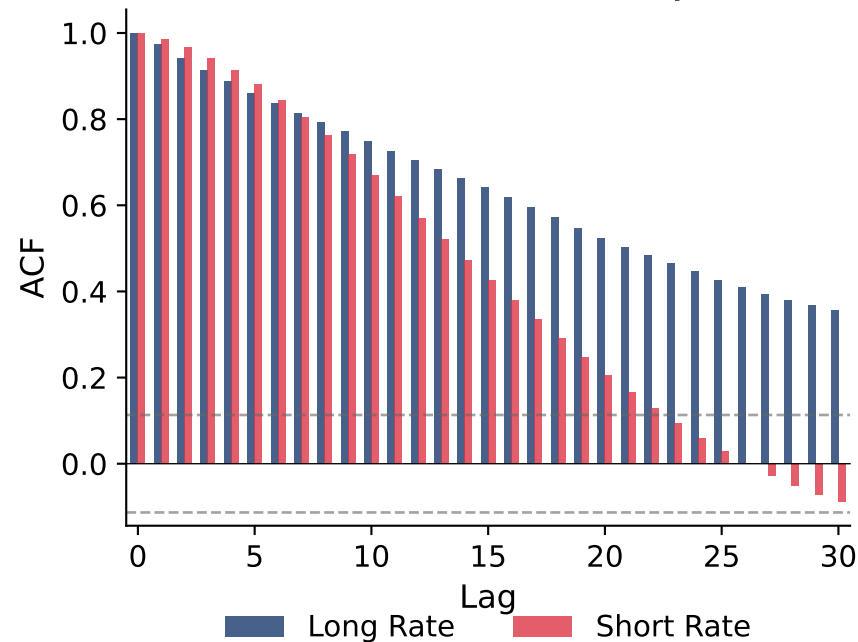
ACF: Levels (Slow Decay)
