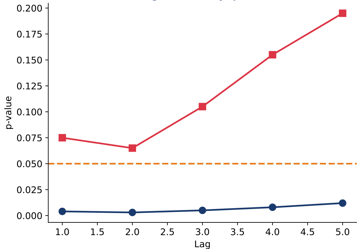
Granger Causality: p-values
