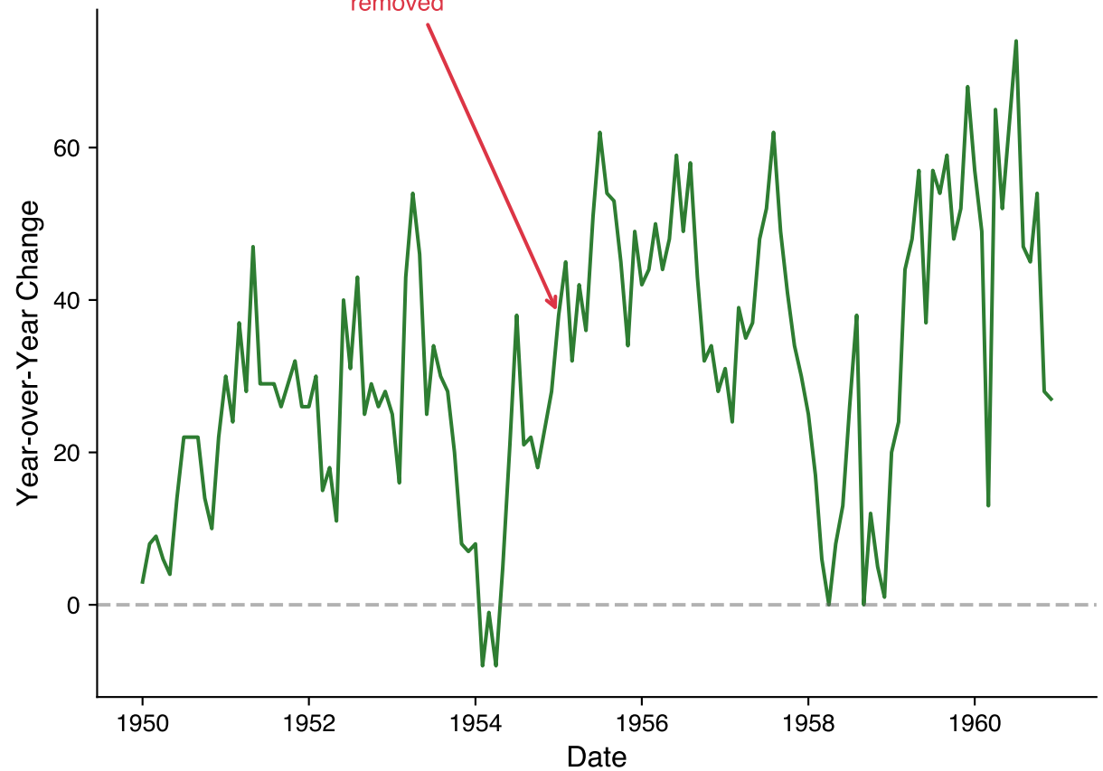
After \Delta_{12} Y_t = Y_t - Y_{t-12} Seasonality removed
