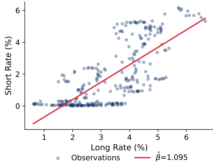
Engle-Granger: Cointegrating Regression
