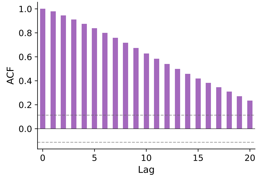
ACF of Residuals
