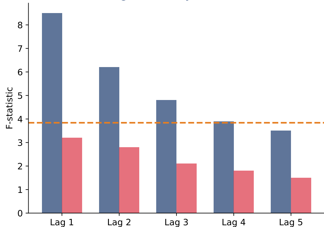
Granger Causality: F-statistics
