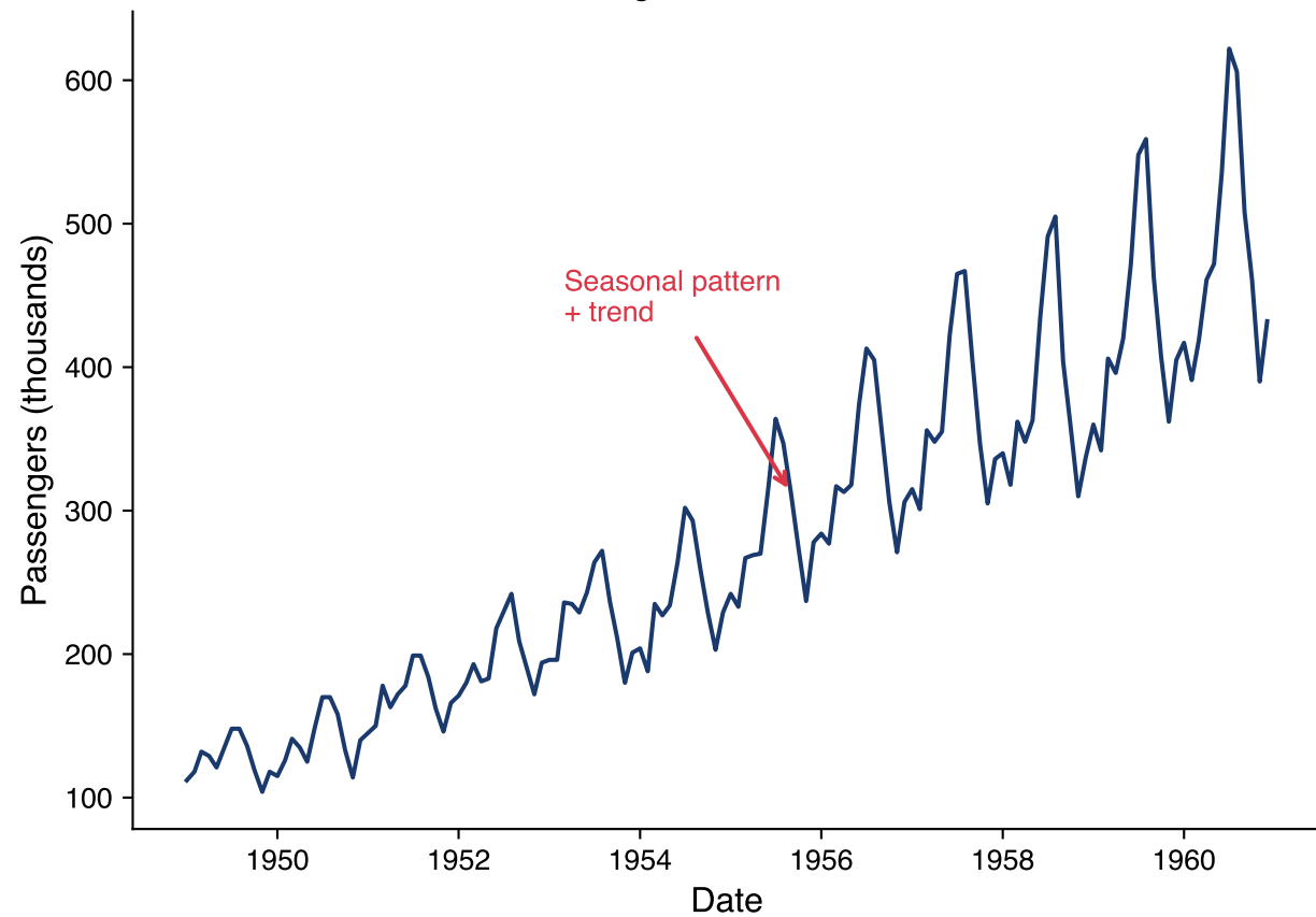
Original Series Y_t
