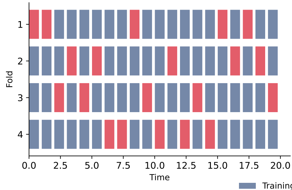
k-fold CV (WRONG) Future leaks into training!
