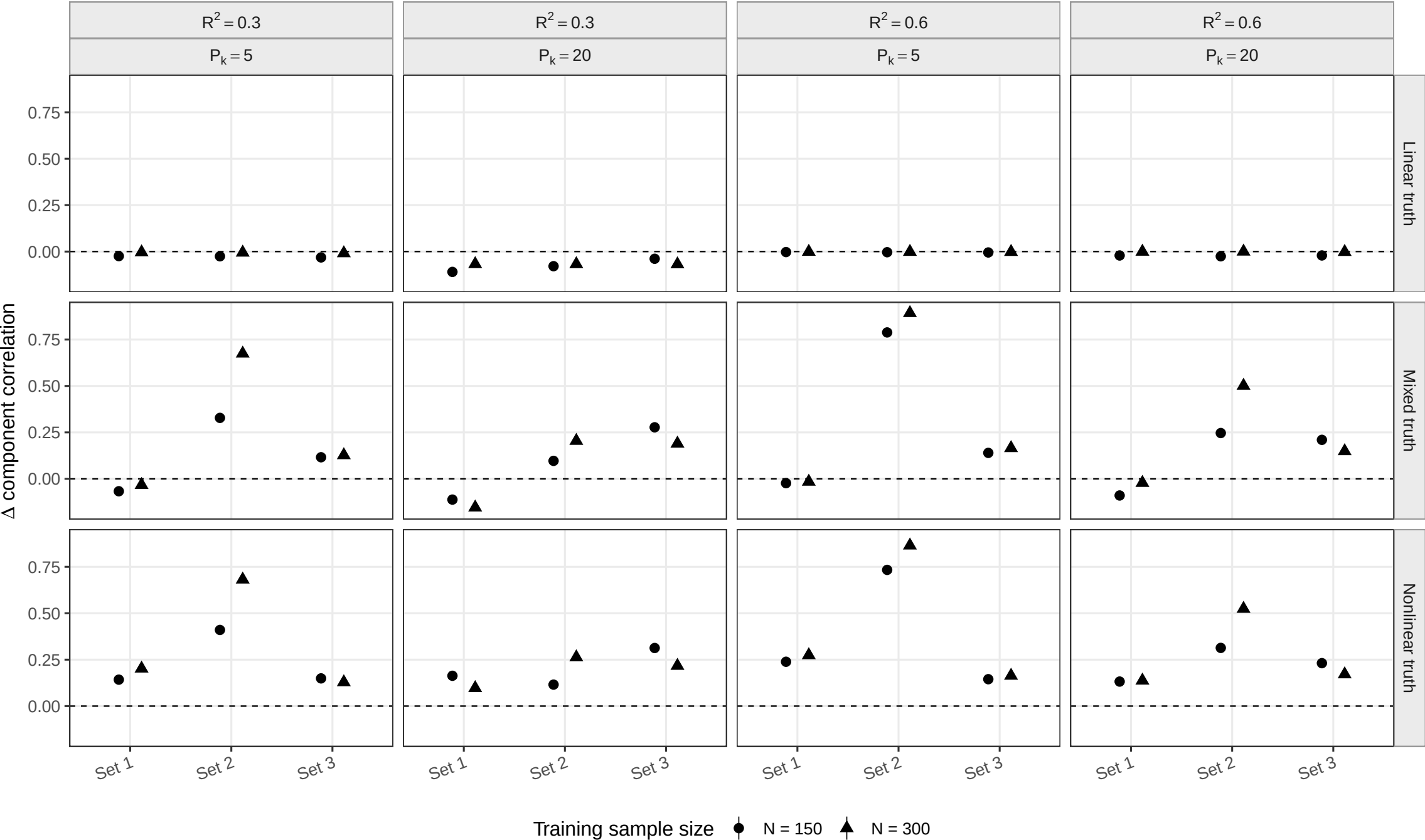
Component recovery by design condition
