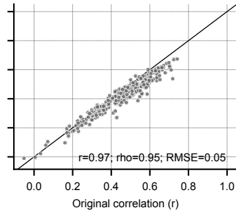
impute = vae_imputed
