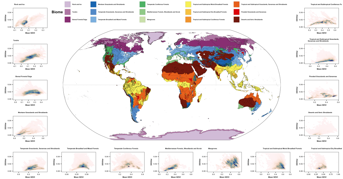
Figure 5: Map of terrestrial biomes along with hex plots of mean NDVI and DENVar for each biome.
