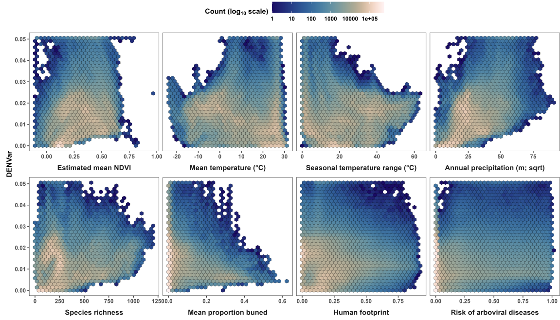
Figure 4: Hex plots of the relationship between the long-term global Dynamic Estimate of NDVI Variance (DENVar) and common ecological metrics. The fill of the hexagonal cells represents the log-10 number of points within the cell. Rowwise, the variables are: long-term mean NDVI (as estimated in this manuscript); mean annual temperature, seasonal temperature range, and annual precipitation (1970-2000) from the work of Fick and Hijmans (2017); IUCN Red List species richness (IUCN, 2025); mean proportion burned (1901-2020; Guo et al., 2025); the human footprint index of Keys et al. (2021); and the risk of dengue, chikungunya, Zika and yellow fever (Lim et al., 2025).
