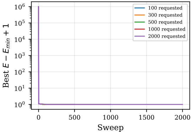
SA convergence (12-var execution QUBO)
