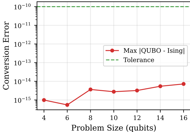
QUBO-Ising Equivalence
