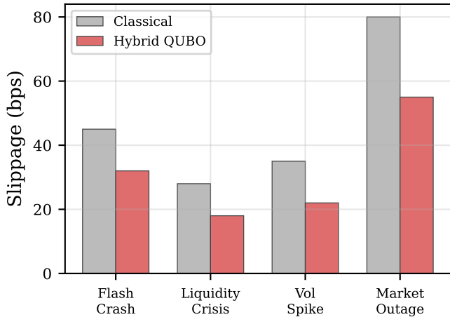
Stress Scenario Slippage
