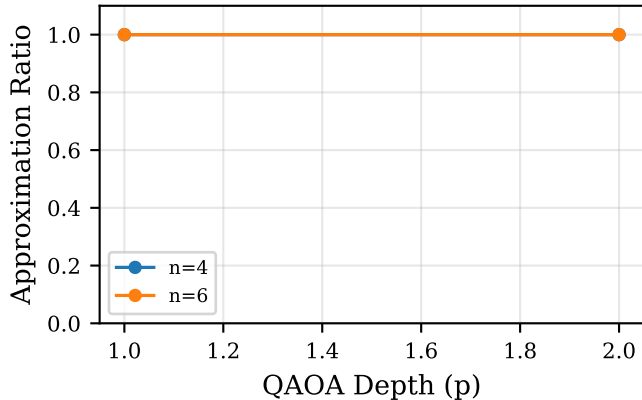
Noisy Simulator
