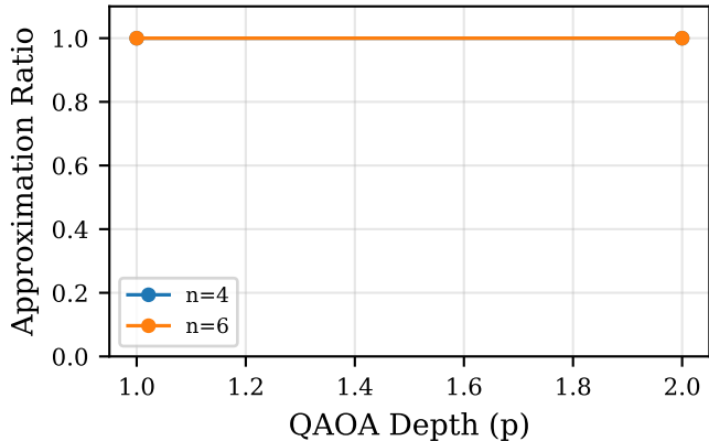
Ideal Simulator
