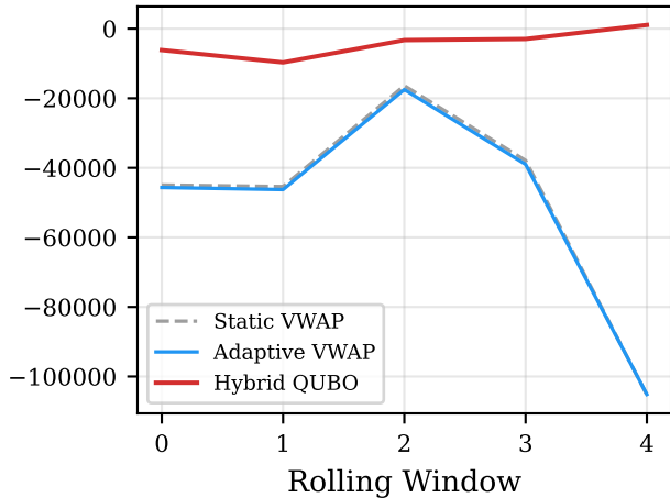
Walk-Forward Analysis
