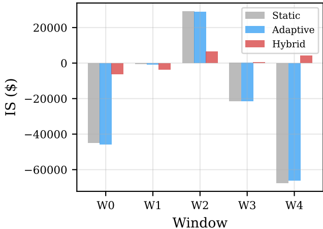
Per-Window Shortfall
