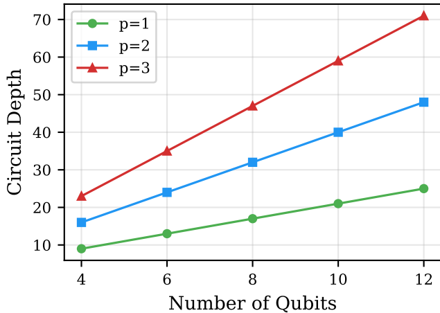
QAOA Circuit Depth
