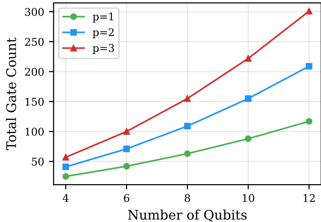
QAOA Gate Count
