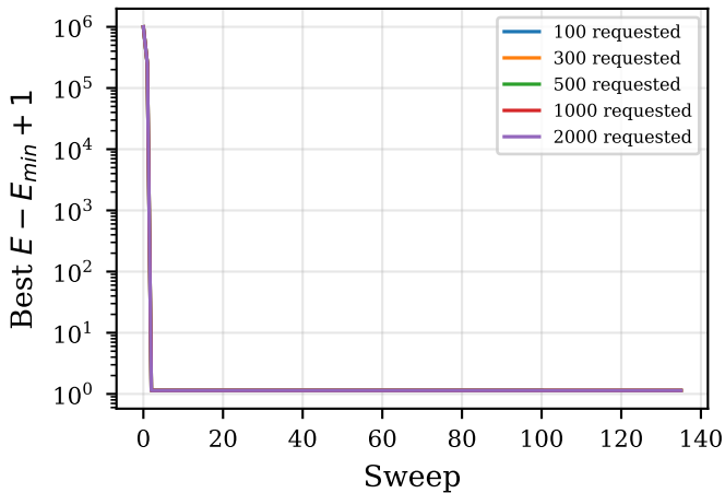
SA convergence (12-var execution QUBO)
