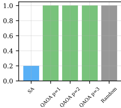
Best-of-shots
