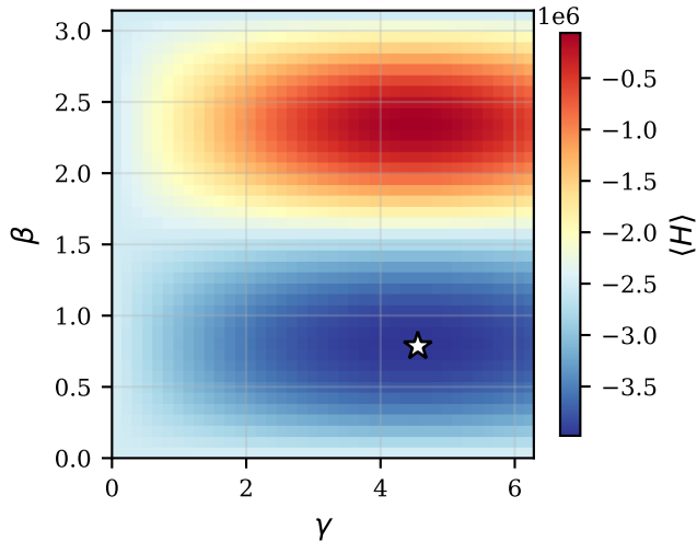
Exact \langle H \rangle , p = 1 , n=4
