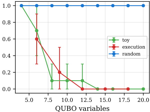
SA success rate (exact reference)
