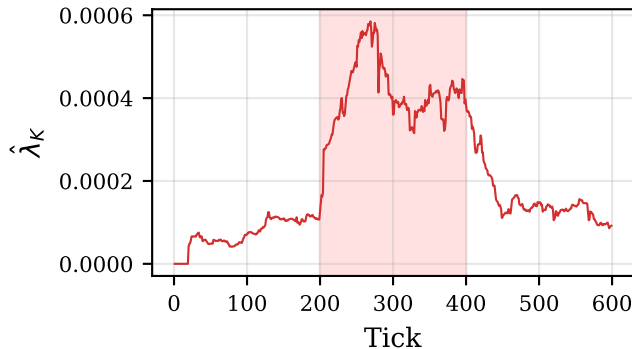
Stress/calm ratio 5.3 [5.1, 5.6] (30 seeds)
