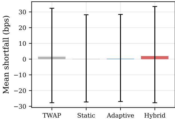
Walk-forward, 30 seeds
