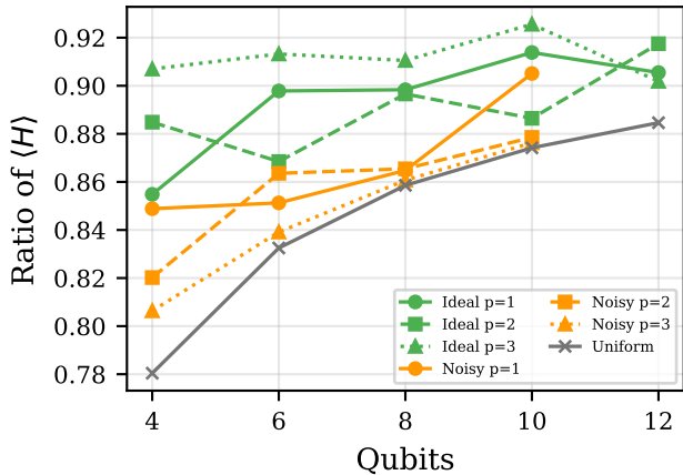
Mean-energy quality
