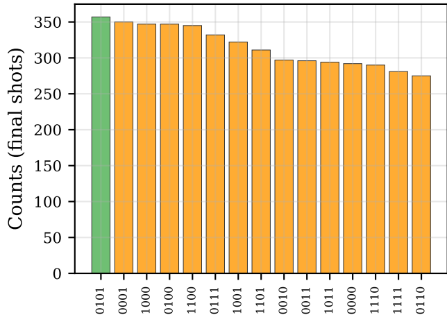
QAOA Noisy, n=4 , p=1 (green = optimal)
