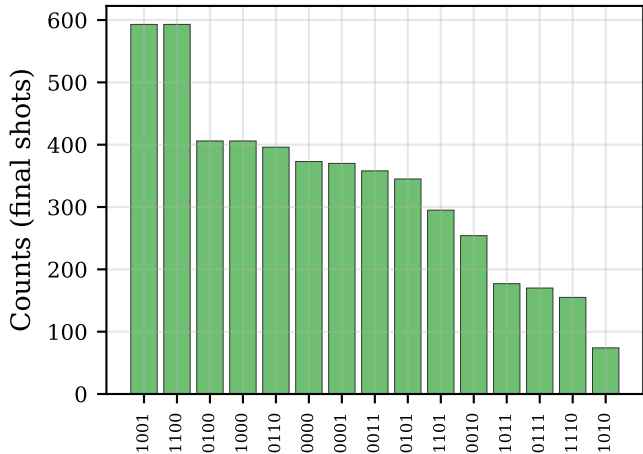
QAOA Ideal, n=4 , p=1 (green = optimal)
