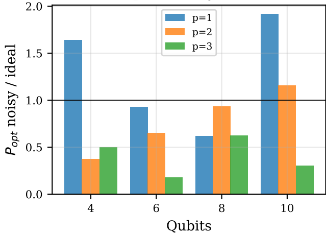
Success probability under noise
