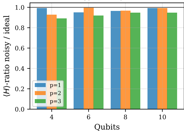
Mean-energy quality under noise
